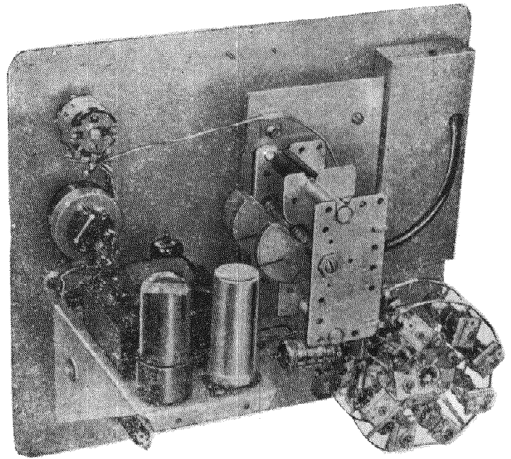
INTERIOR VIEW SHOWING RF TURRET CONSTRUCTION
